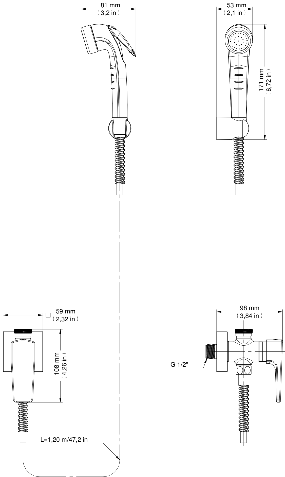
DUCHA HIGIENICA COM REGISTRO E DERIVAÇÃO LIFT - CHROME LIFT TOILET HANDSHOWER W/ VALVE AND OUTLET FOR TOILET TANK - 1/2" - CHROME DUCHA HIGIENICA CON LLAVE Y DERIVADOR LIFT - CHROME
